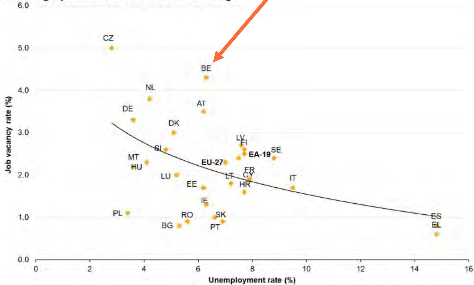
Beveridge points, 2021Q1-2021Q4 average
